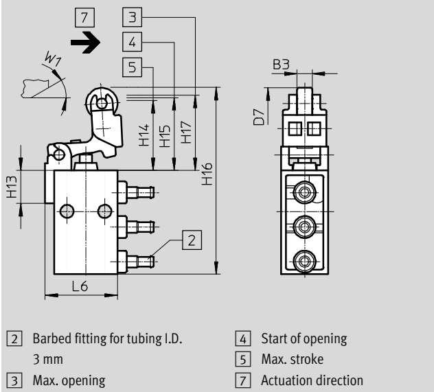
Roller lever valve with idle return L/O-3-PK-3
