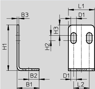
Mounting bracket HV-M5
