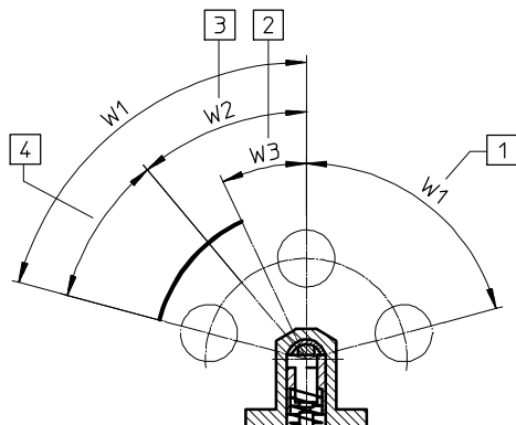
Valve components 1 and 2 turned 180° around the longitudinal axis
