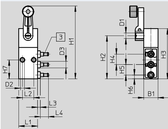
Swivel lever valve RW/O-3-PK-3
