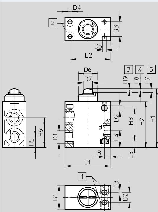
Stem actuated valve V-3-1/4-B, VO-3-1/4-B
