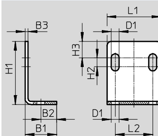
Mounting bracket HV-1/8
