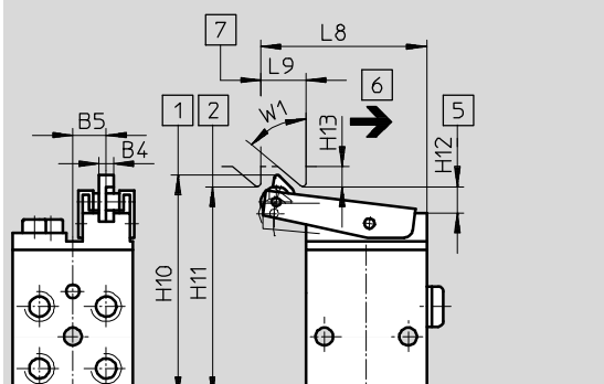
Toggle lever valve LS-4-1/8
