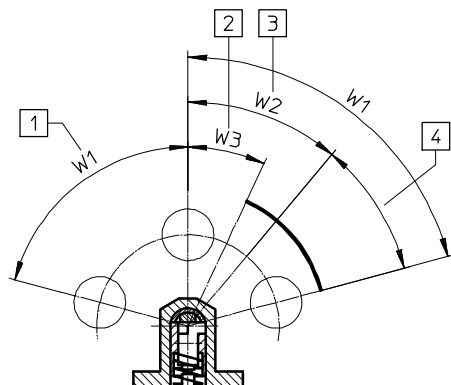
Valve components 1 and 2 turned 180° around the longitudinal axis
