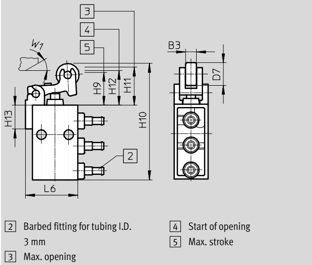
Roller lever valve R/O-3-PK-3
