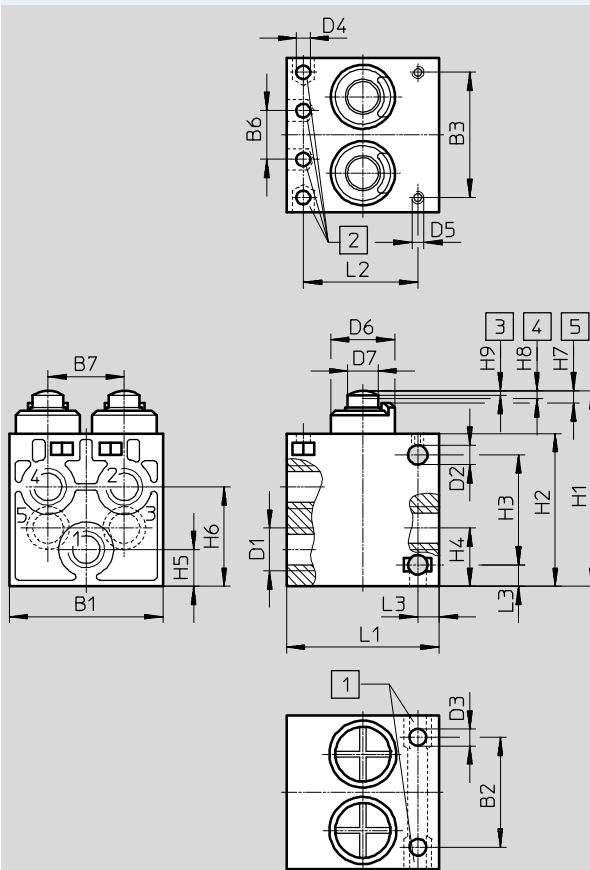
Stem actuated valve V-5-1/4-B
