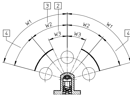
Valve components 1 and 2 turned 90° around the longitudinal axis
