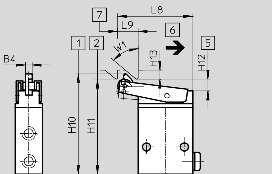
Toggle lever valve LS-3-1/8, LOS-3-1/8
