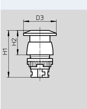
Mushroom pushbutton P
