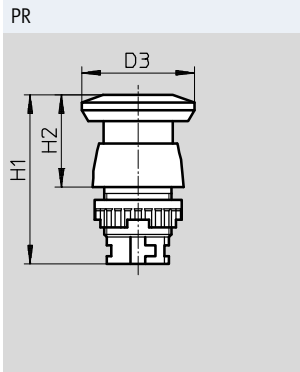
Mushroom pushbutton with detent PR
