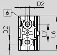
SDE5 with wall bracket
