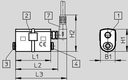
SDE5-...-K, cable version
