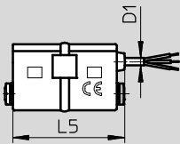
SDE5-...-K, cable version
