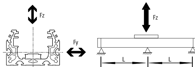
Force Fz
