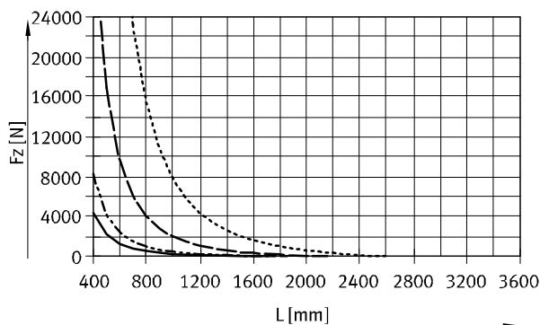
Force Fz
