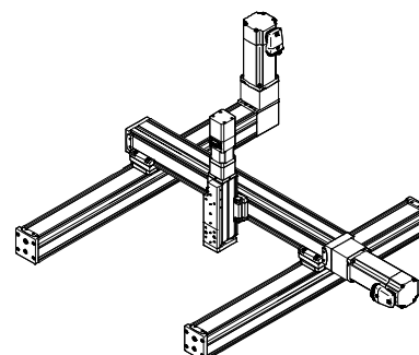
Three-dimensional gantry
