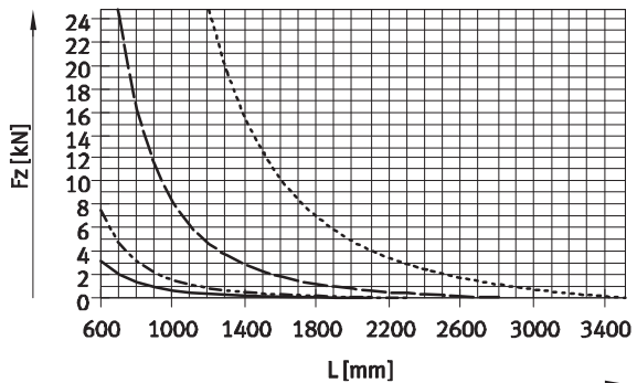
Force F_z
