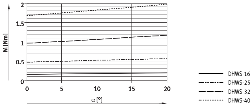
Determination of the actual gripping torques M_{Grtotal} for DHWS-...-NC as a function of application
