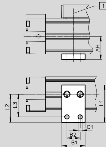
DGC-K-18/25 with MUP-18/25-P (for mounting on one side)
